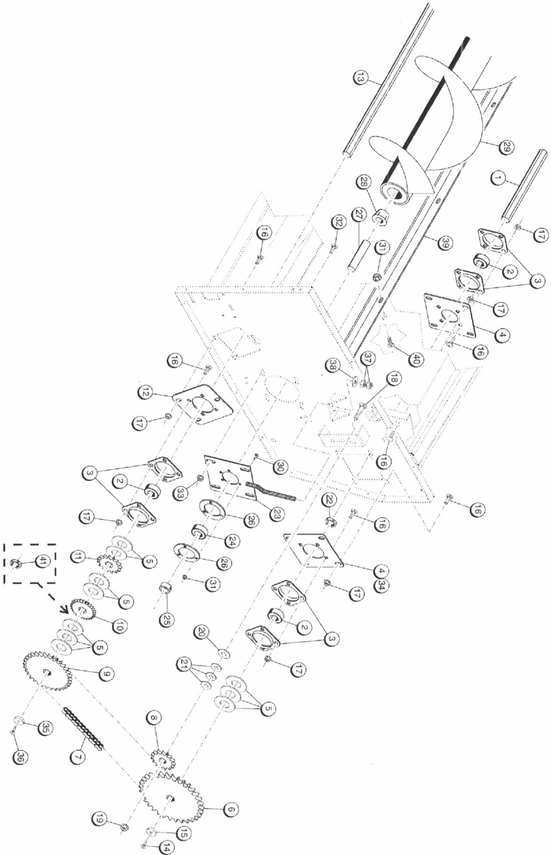
SHAFT DRIVEN CORN HEAD DRIVES, L.H. SIDE
